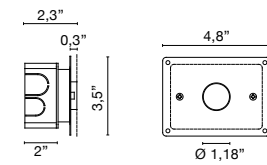
Kit: box + perforated plaster Kit: caja + yeso perforado
