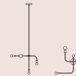
Baubien Suspension L 23 x W 24 x H 17.5 in L 580 x W 640 x H 448 mm Total height variable
