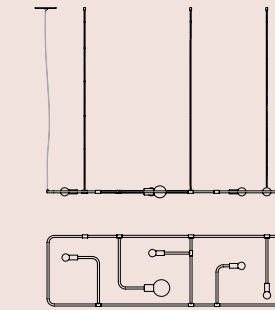
Baubien (ceiling) L 60 x W 17 in L 1524 x W 432 mm Height variable
