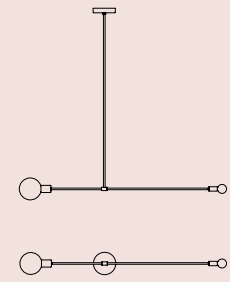
Antipode L 47 x W 4 x H 4 in L 1194 x W 100 x H 100 mm Total height variable
