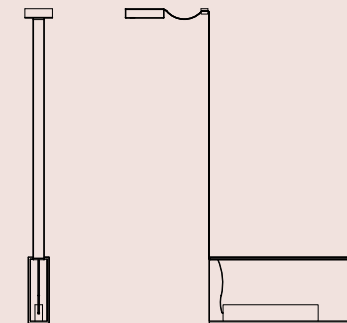
Sainte 09 L 27 x W 3.8 x H 12 in L 686 x W 96 x H 305 mm Total height variable
