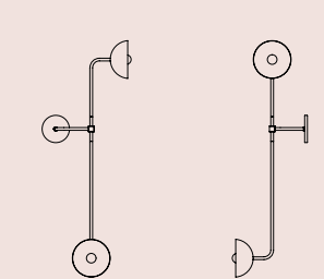
Baubien Wall Double Shade L 16 x W 14 x H 42 in L 406 x W 356 x H 1118 mm
