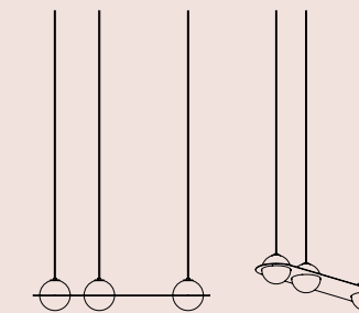
Laurent 07 L 31 x W 8 x H 5.5 in L 790 x W 200 x H 140 mm Total height variable
