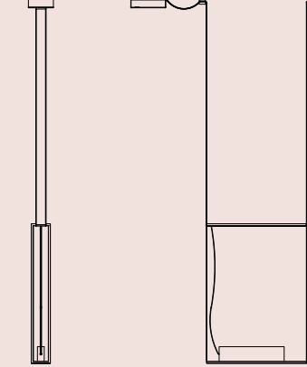
Sainte 08 L 20 x W 3.8 x H 28 in L 510 x W 96 x H 710 mm Total height variable
