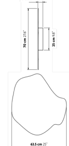
Ya-Ya 70 Wall / Ceiling
