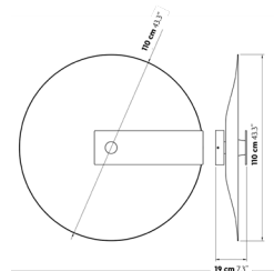
Meridiana 110 Wall / Ceiling
