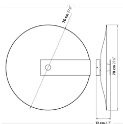
Meridiana 70 Wall / Ceiling
