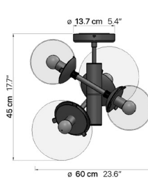
Global 4-Light C
